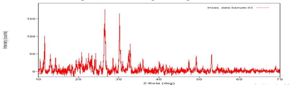
Figure 9: X-RD of crushed tablet
